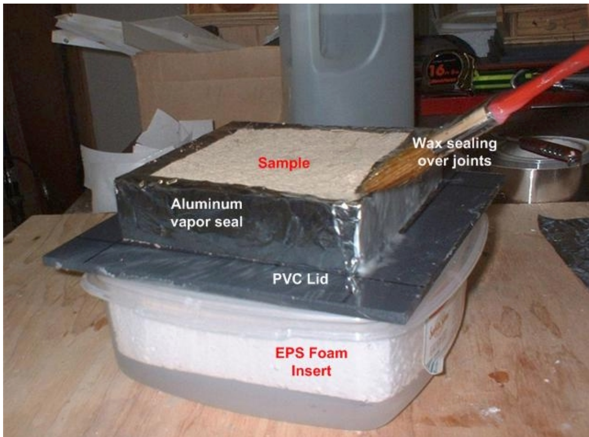
Figure 4.2: Photograph of Sample Assembly
